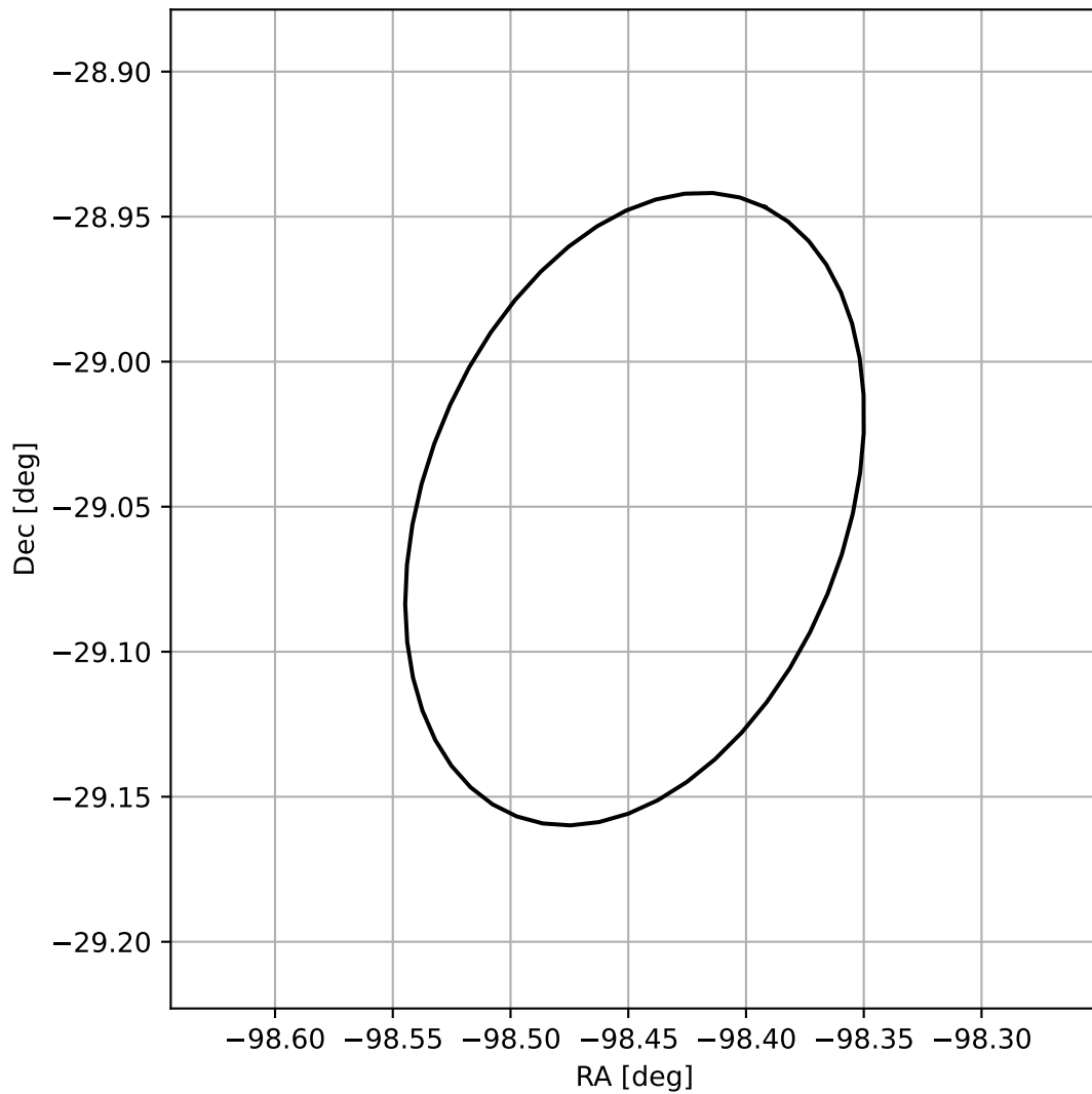
4FGL J1726.2-2903
