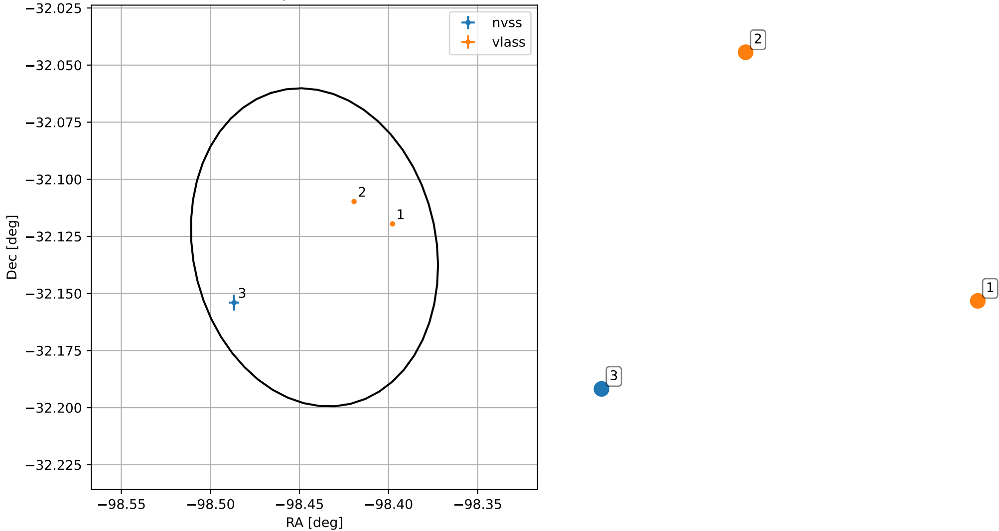
4FGL J1726.2-3207
