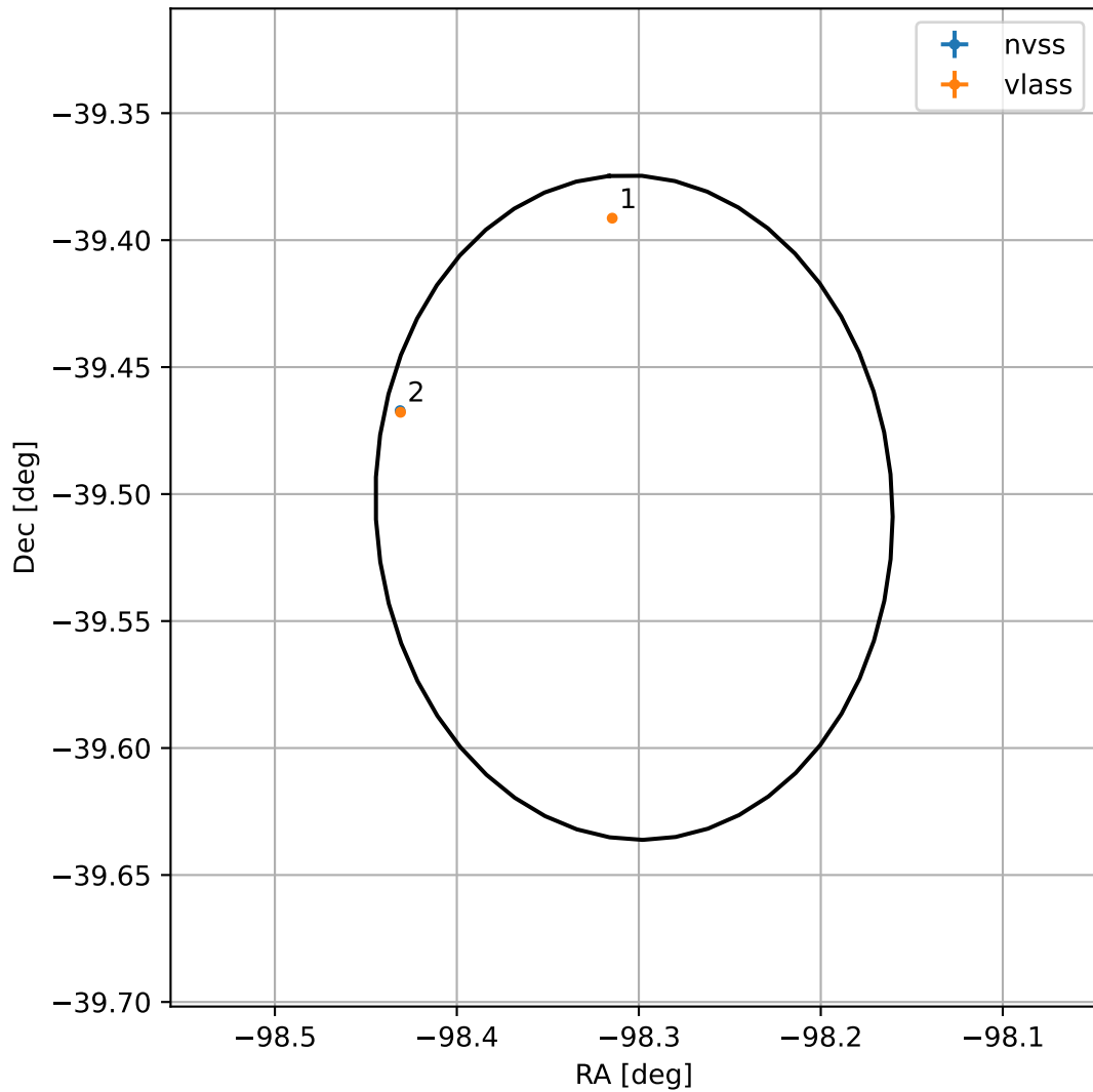
4FGL J1726.7-3930
