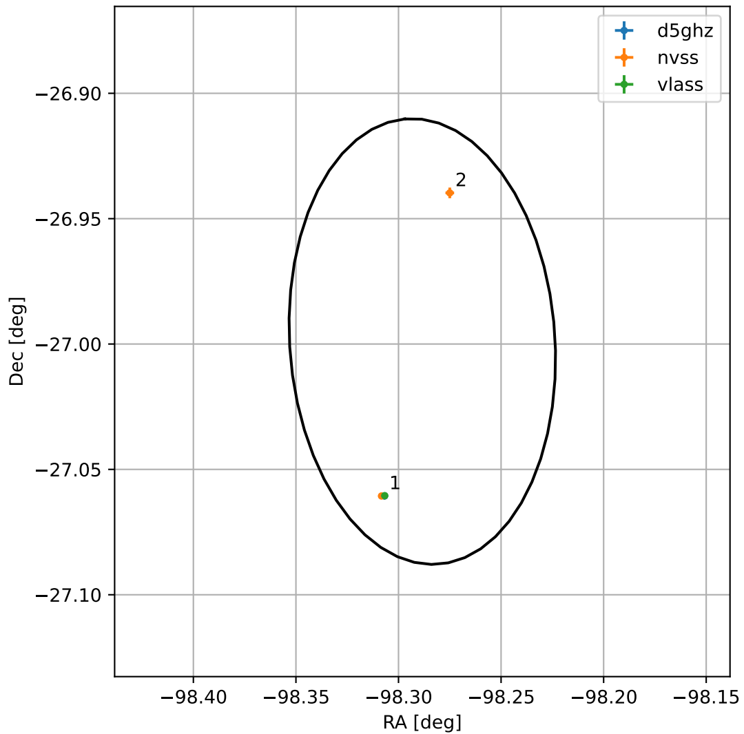
4FGL J1726.8-2659
