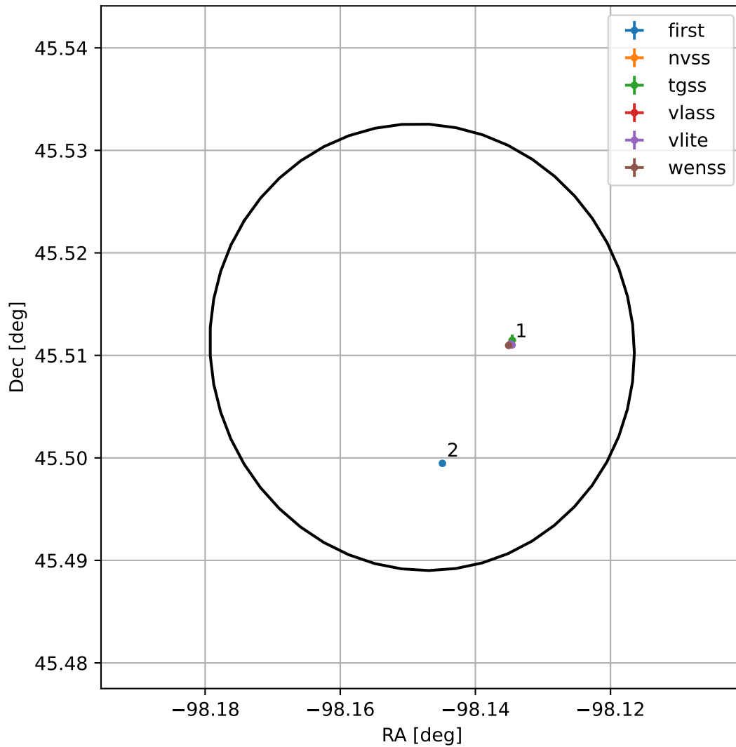
4FGL J1727.4+4530
