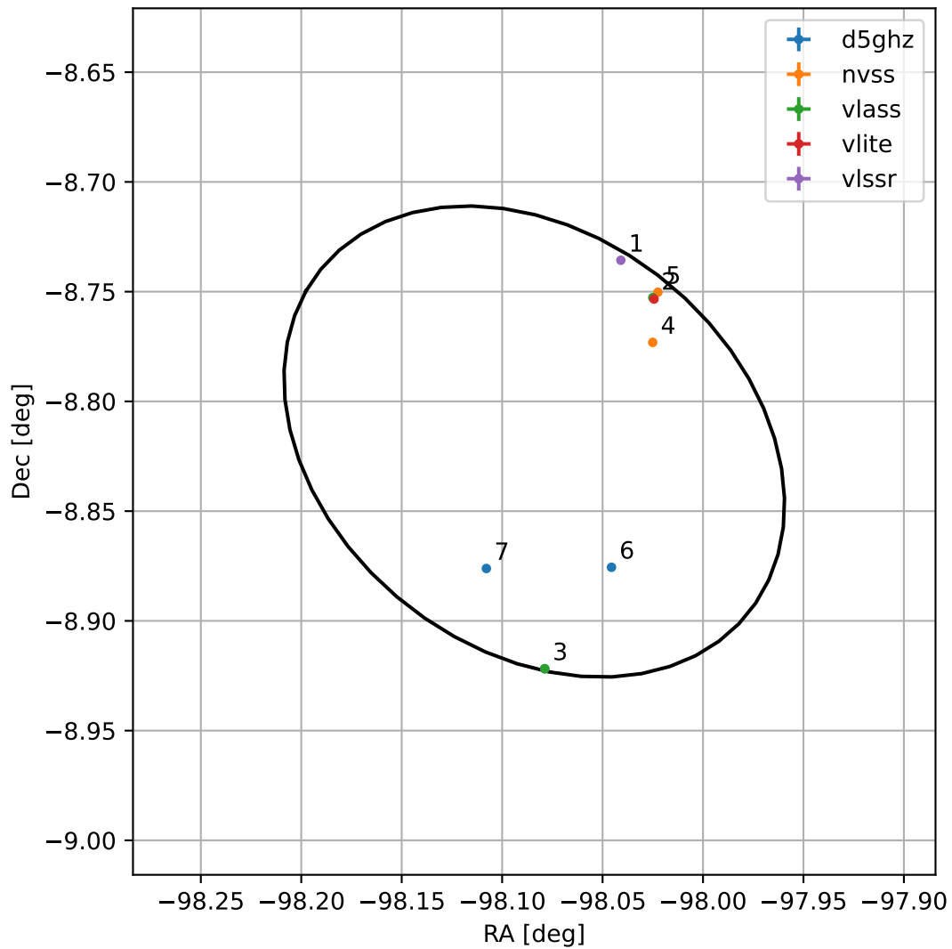
4FGL J1727.6-0849
