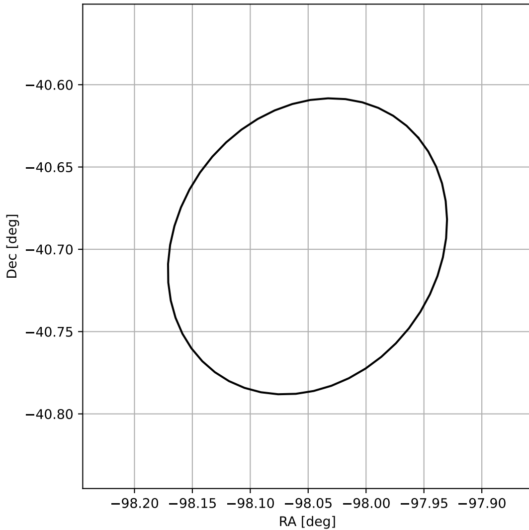
4FGL J1727.7-4041
