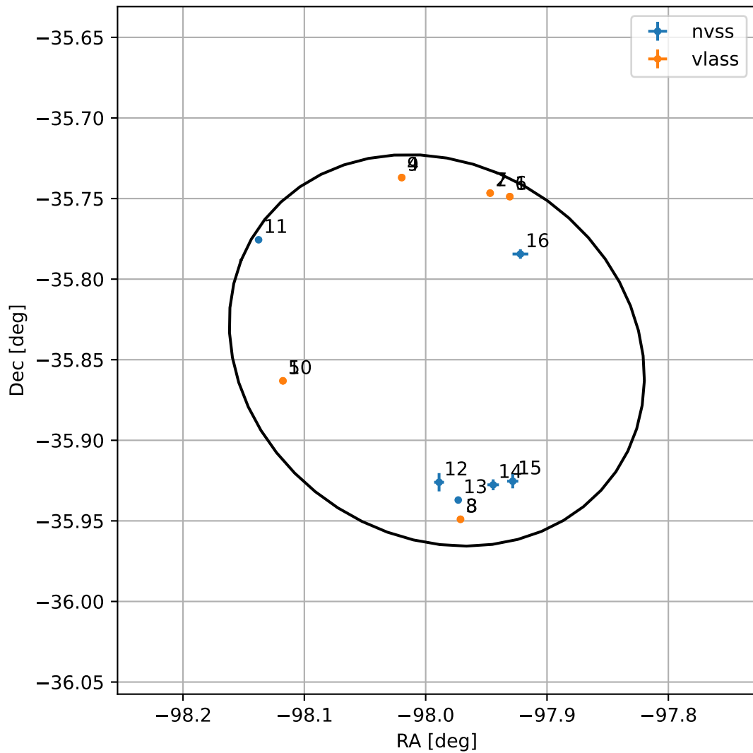
4FGL J1728.0-3550
