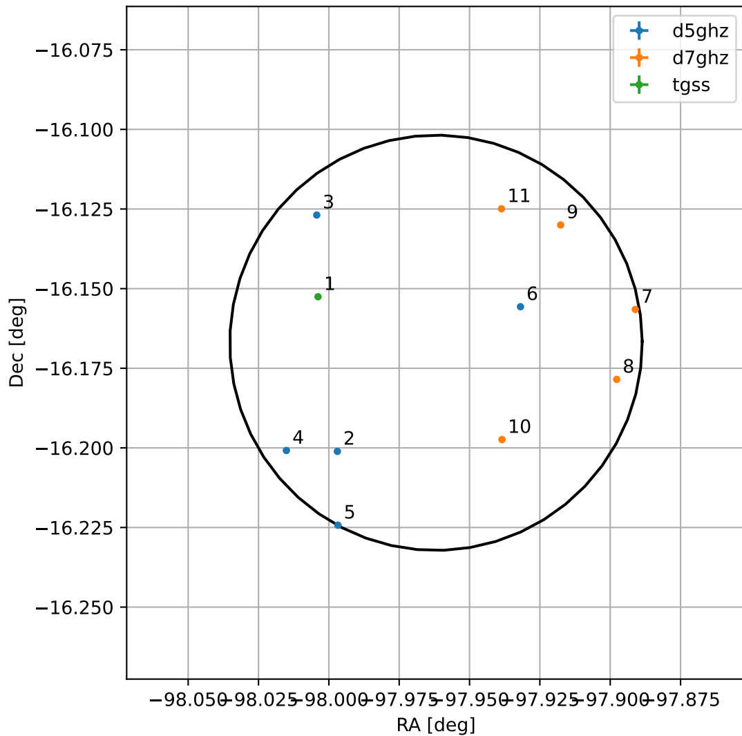
4FGL J1728.1-1610
