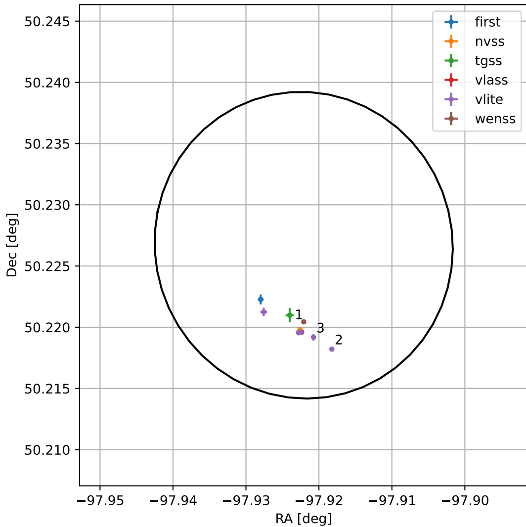
4FGL J1728.3+5013
