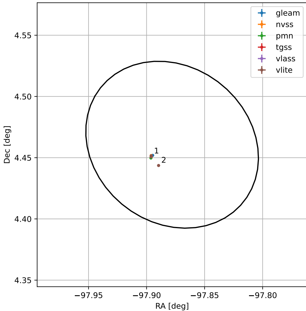
4FGL J1728.4+0427
