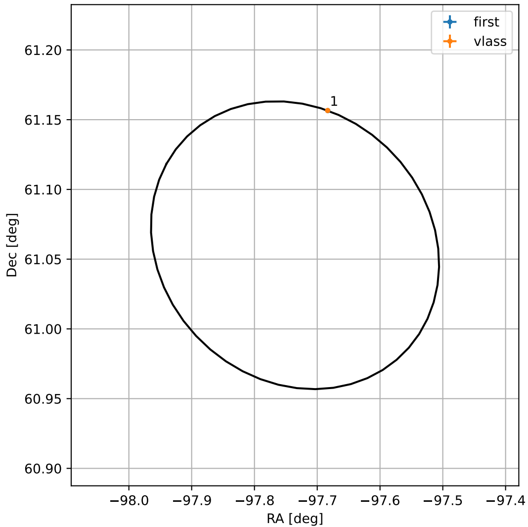
4FGL J1729.0+6103
