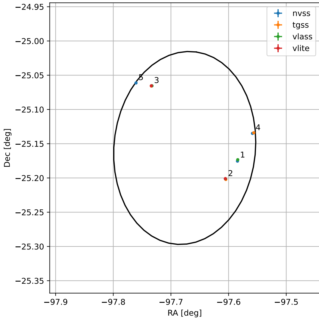
4FGL J1729.2-2509
