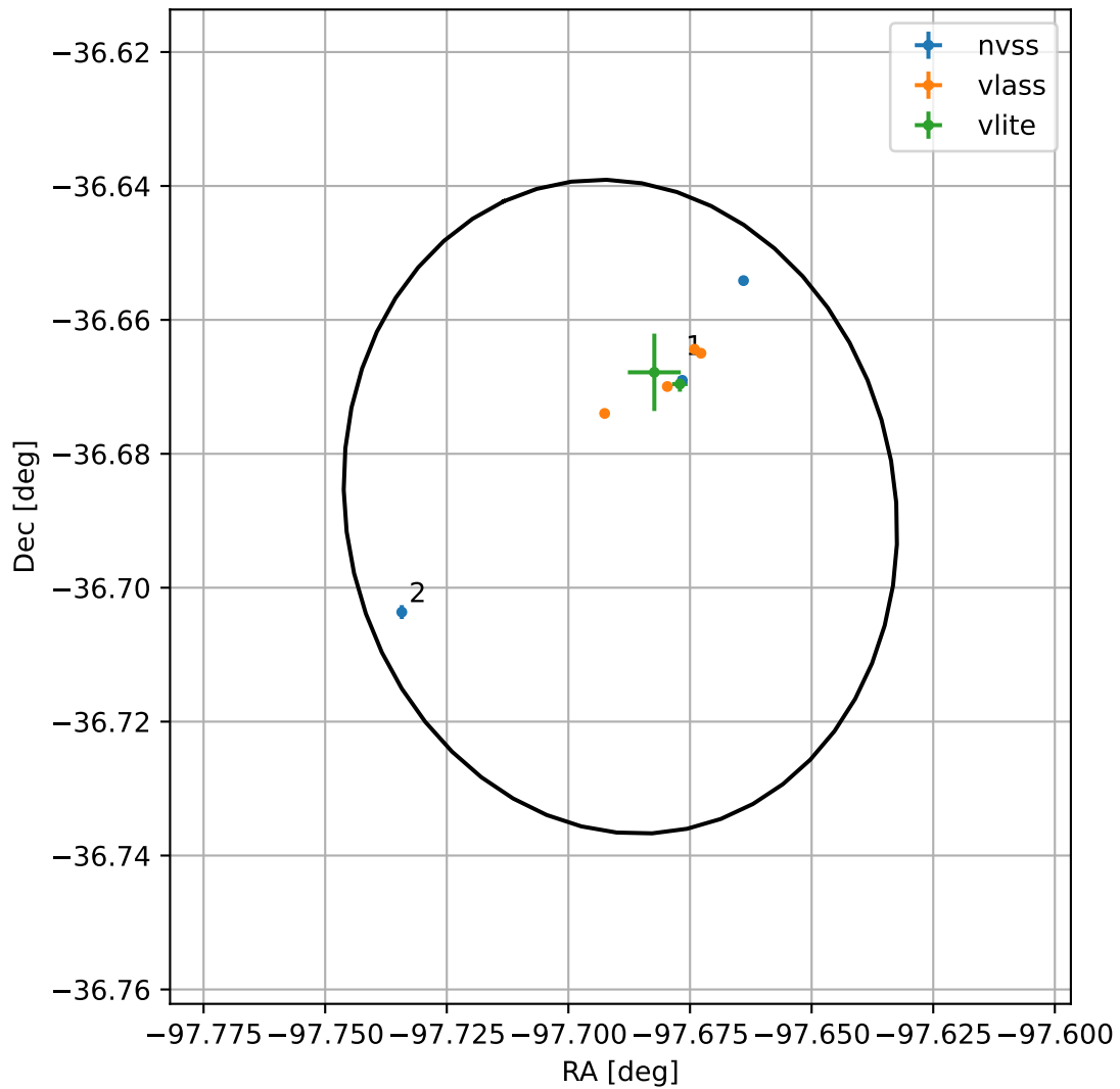
4FGL J1729.2-3641
