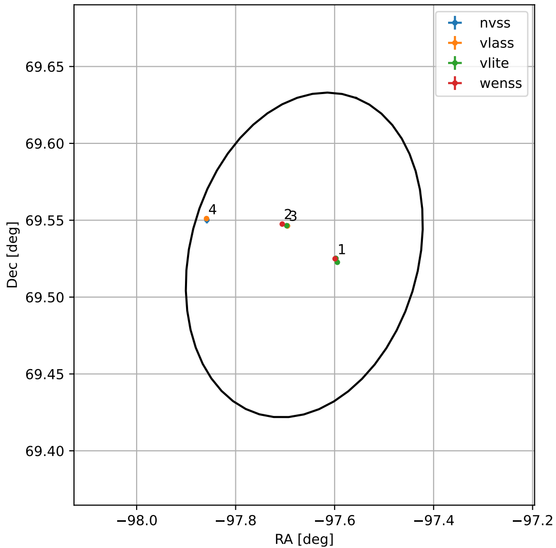
4FGL J1729.3+6931
