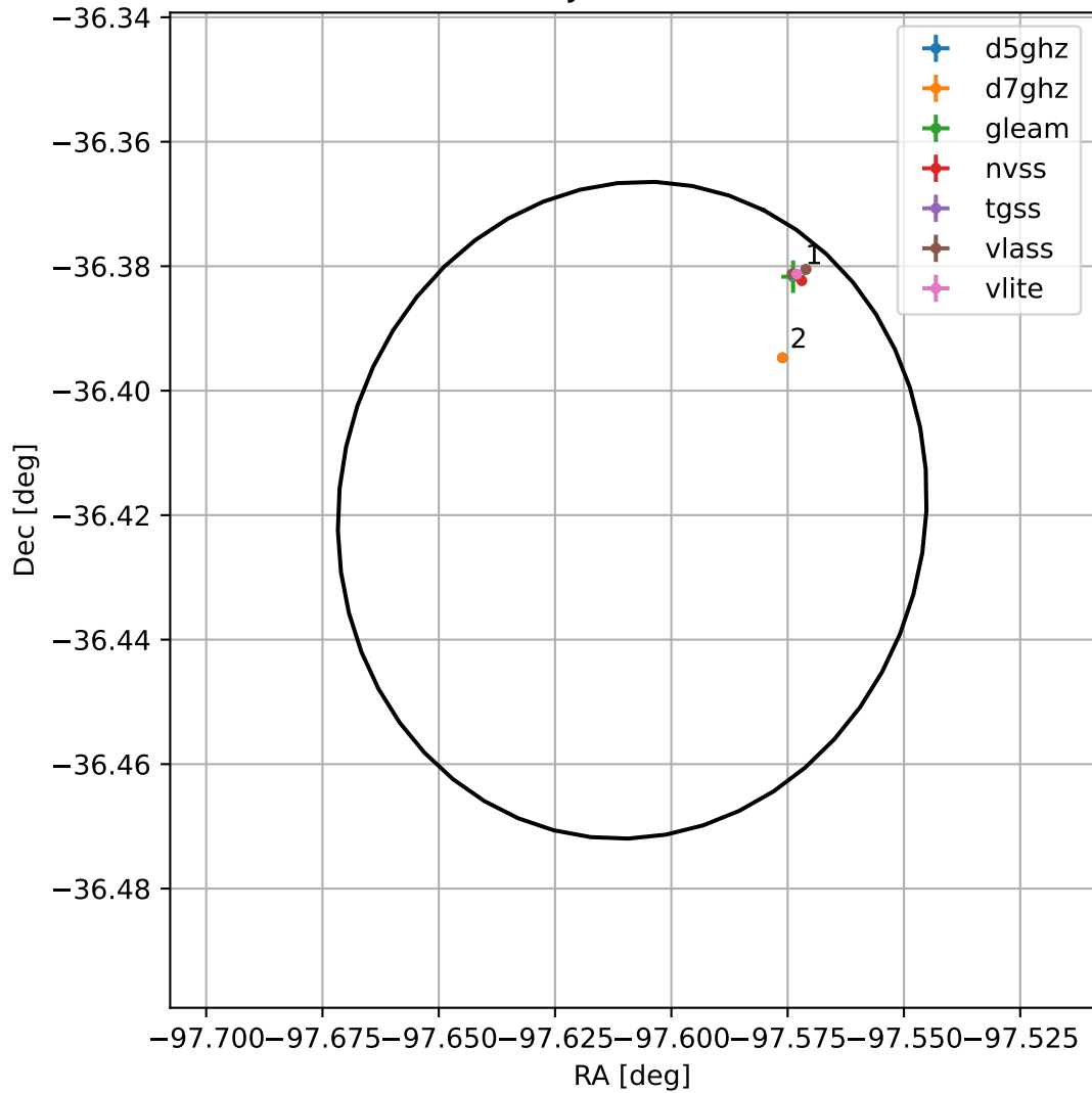
4FGL J1729.5-3625
