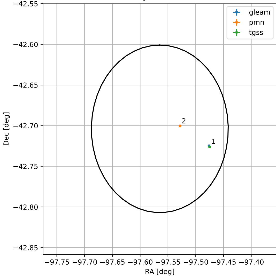
4FGL J1729.7-4242
