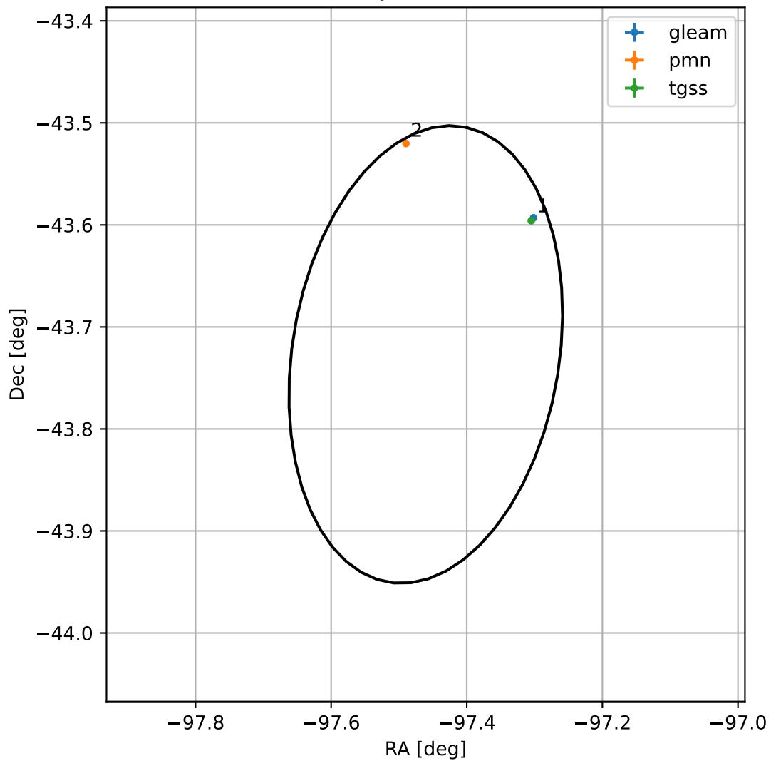
4FGL J1730.1-4343
