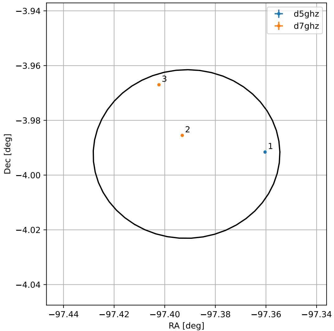
4FGL J1730.4-0359
