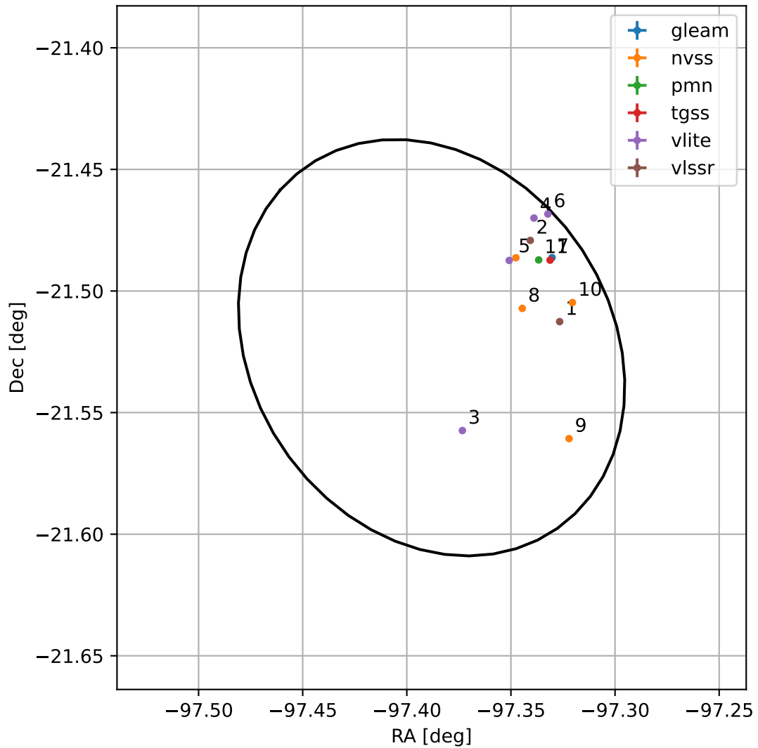
4FGL J1730.4-2131
