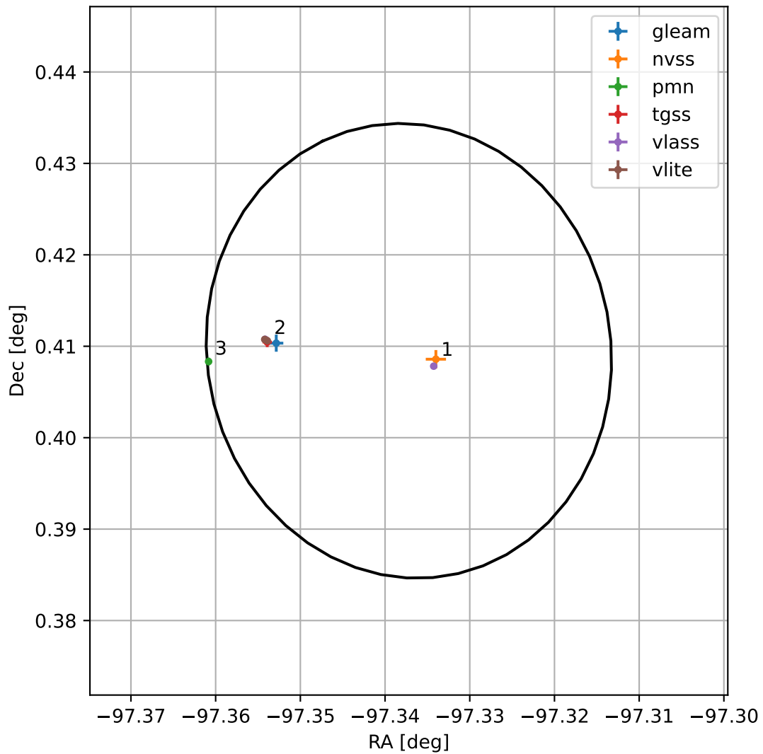
4FGL J1730.6+0024
