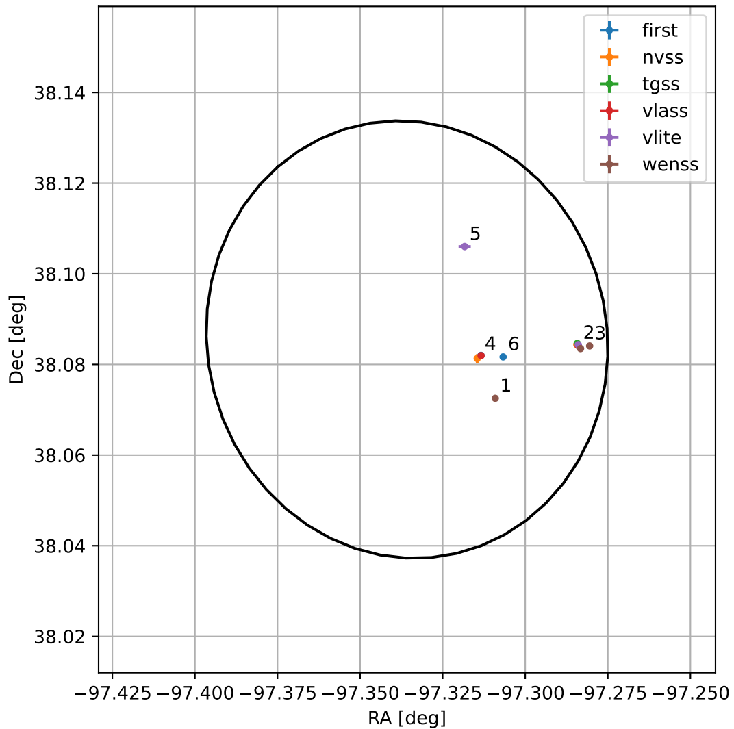
4FGL J1730.6+3805
