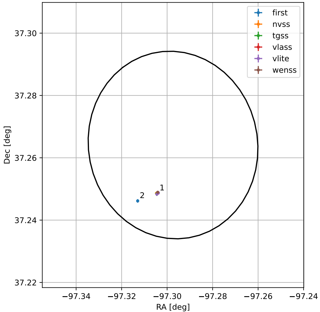
4FGL J1730.8+3715
