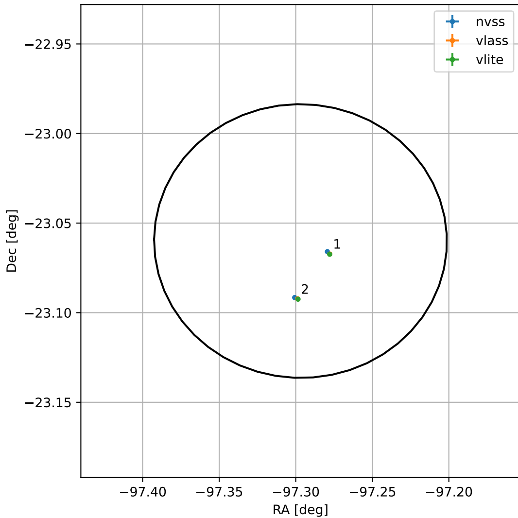
4FGL J1730.8-2303
