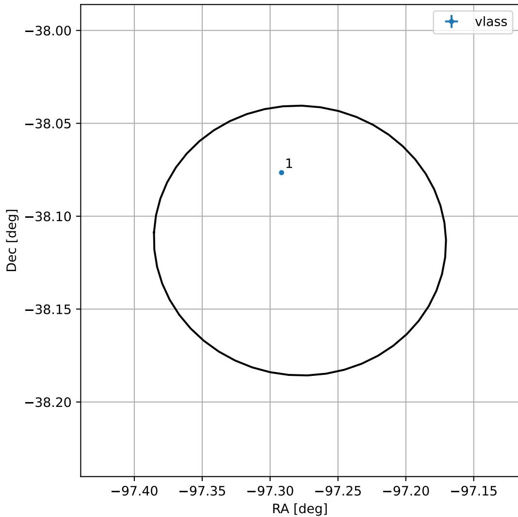
4FGL J1730.8-3806
