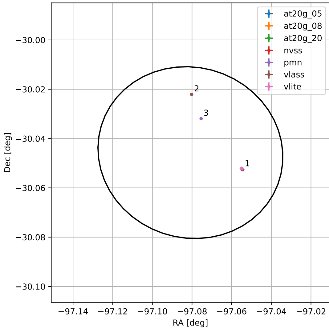
4FGL J1731.6-3002
