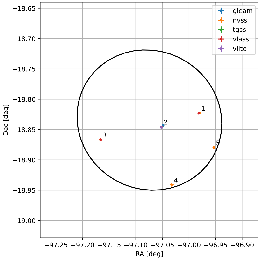
4FGL J1731.7-1850
