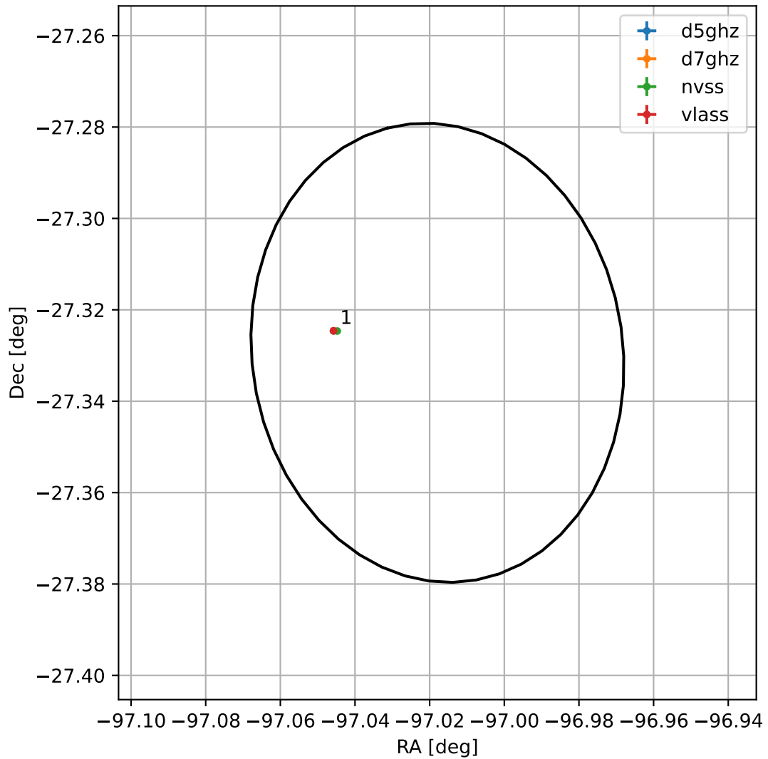
4FGL J1731.9-2719
