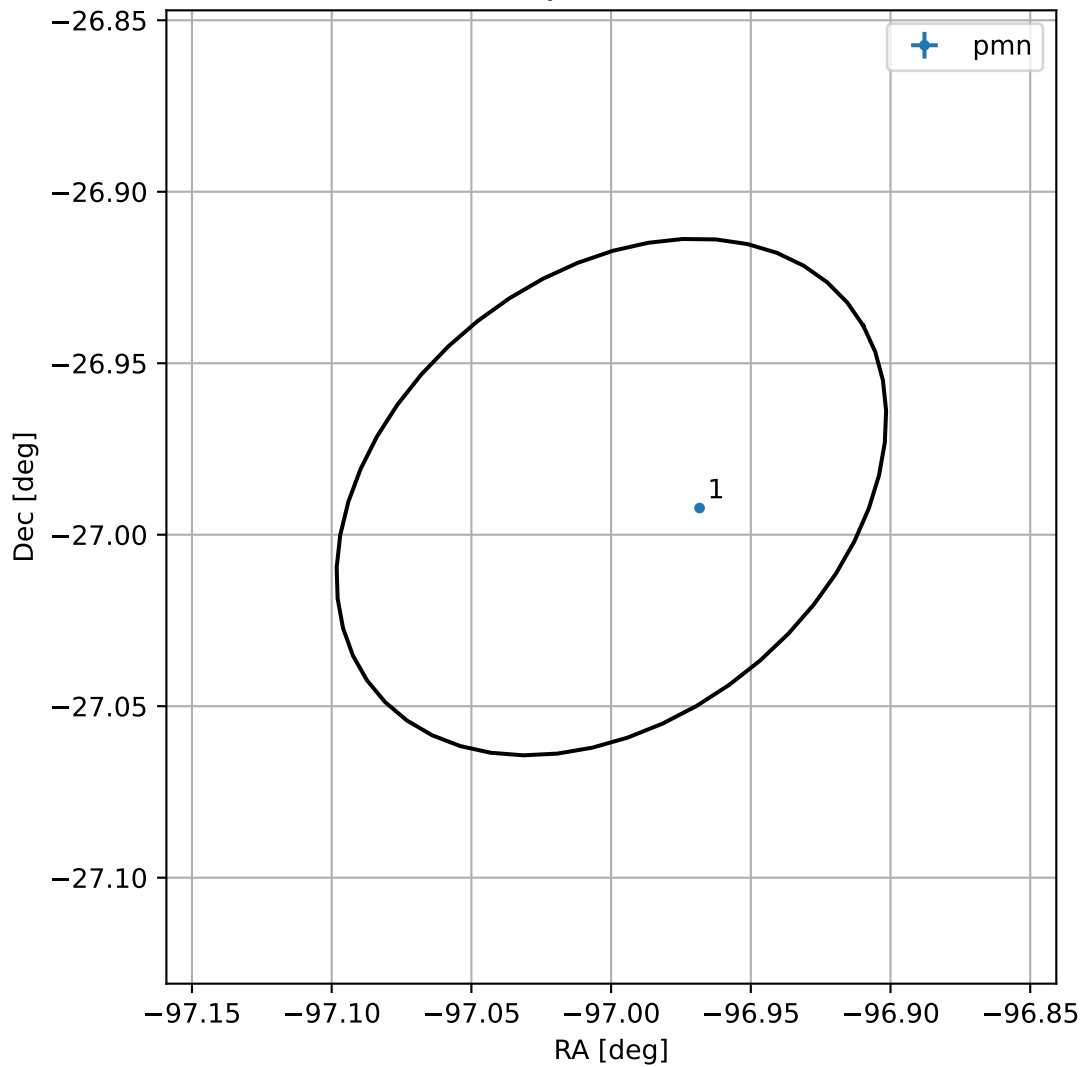
4FGL J1732.0-2659
