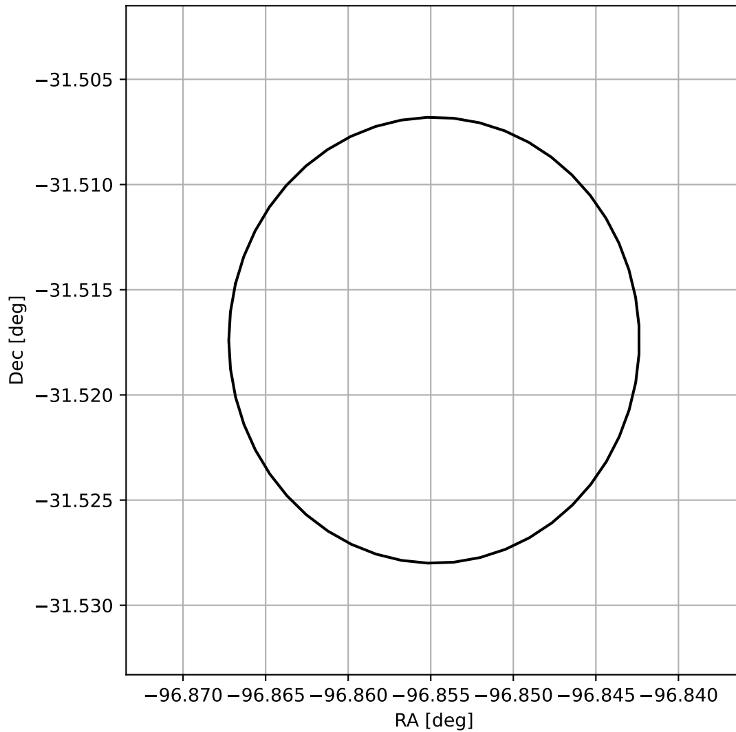
4FGL J1732.5-3131
