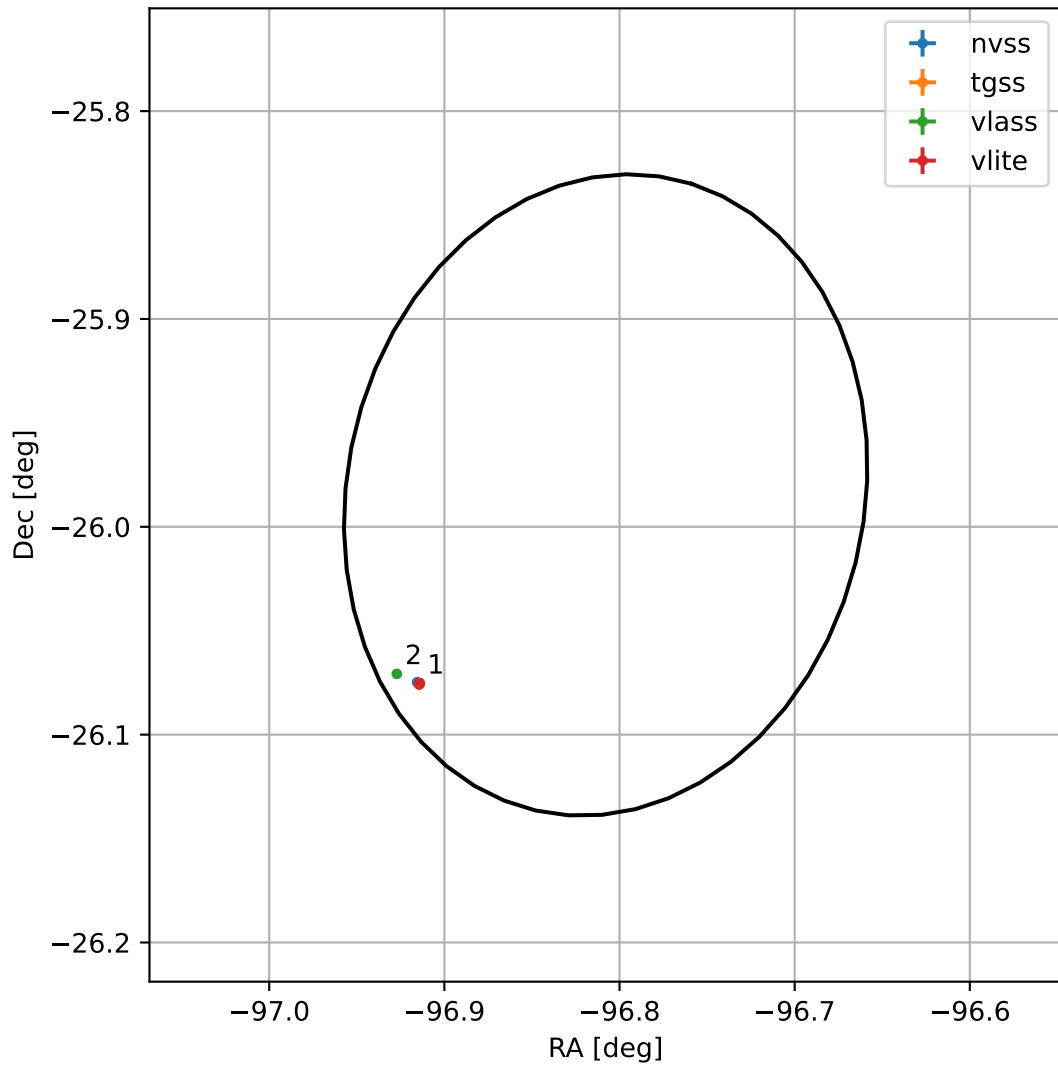
4FGL J1732.7-2559
