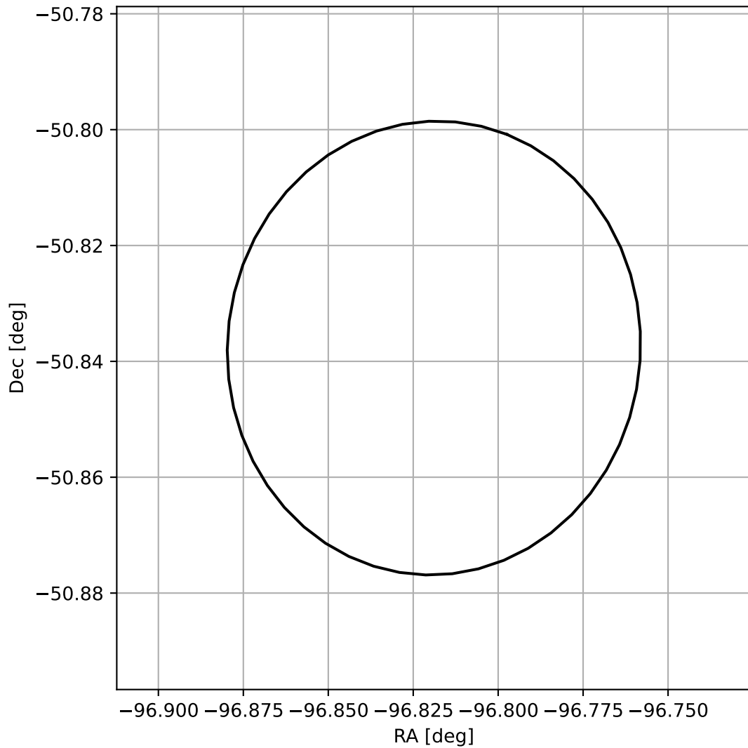
4FGL J1732.7-5050
