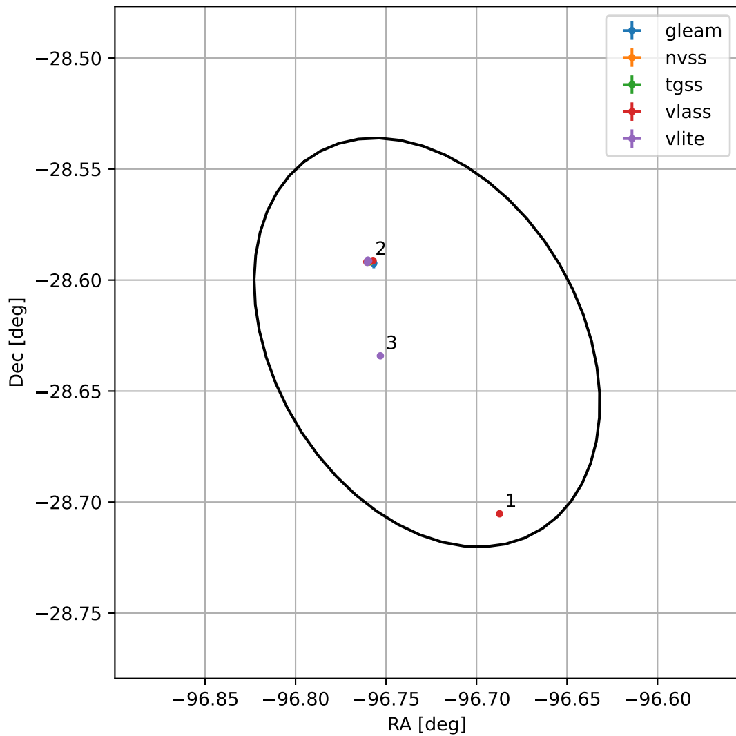
4FGL J1733.0-2837
