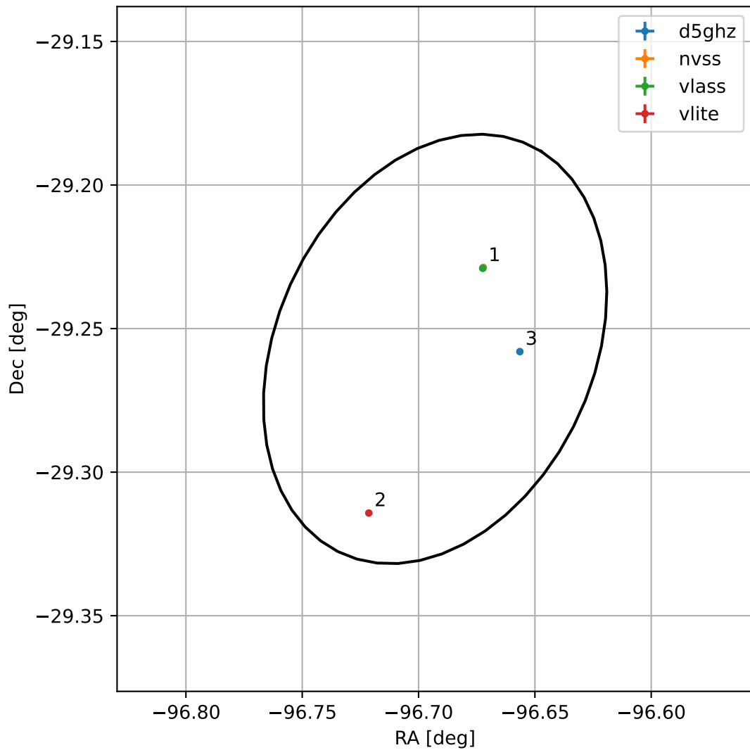
4FGL J1733.2-2915
