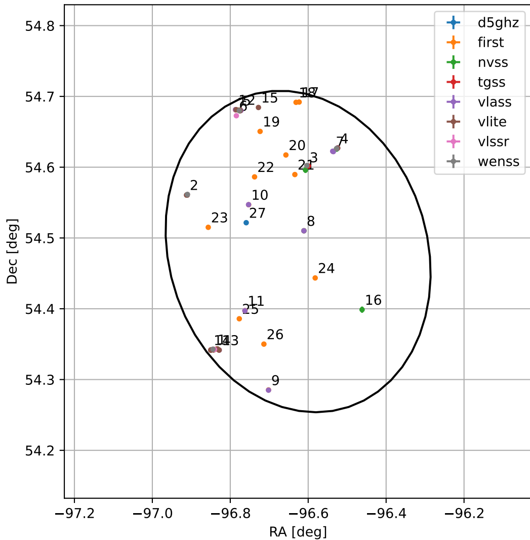
4FGL J1733.4+5428
