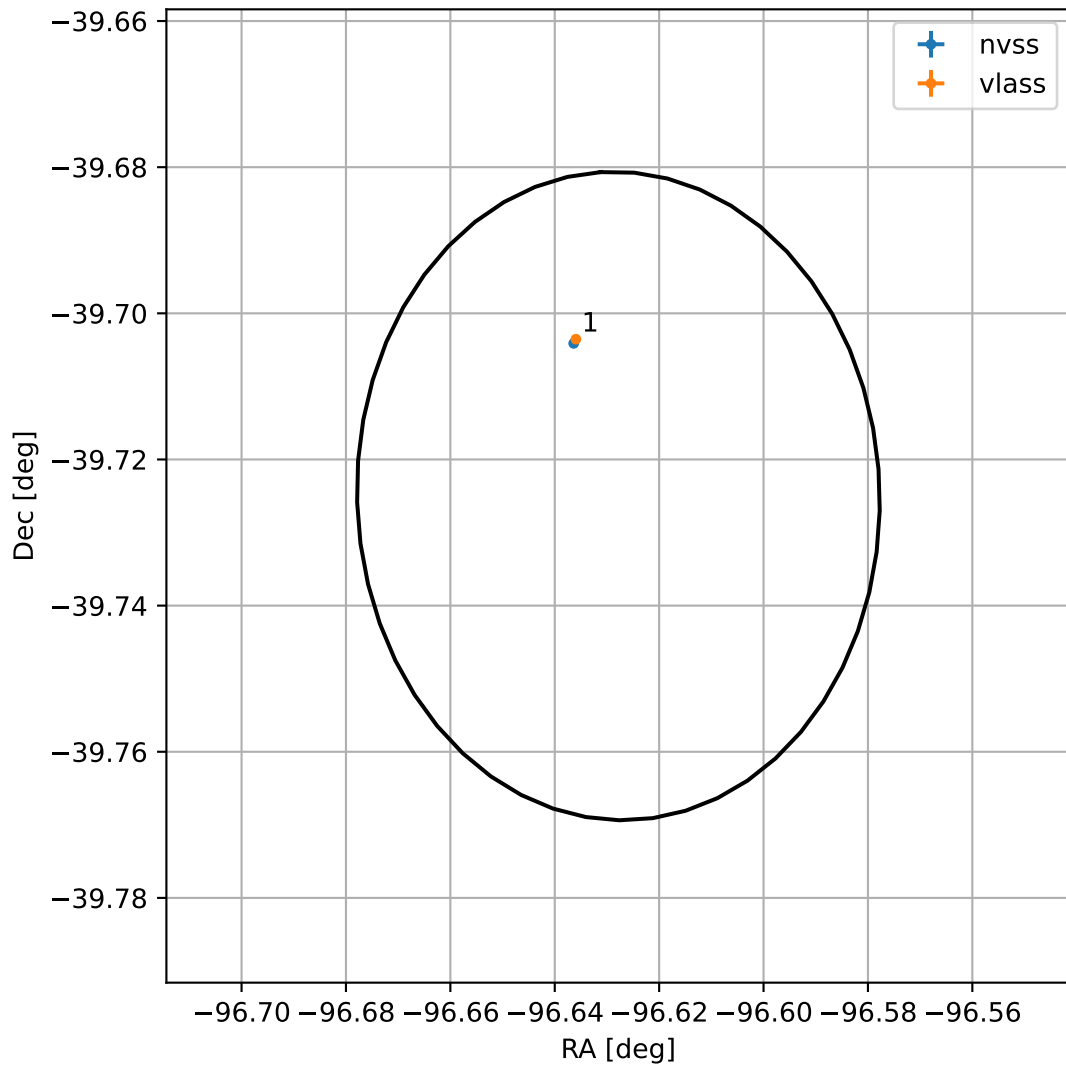
4FGL J1733.4-3943
