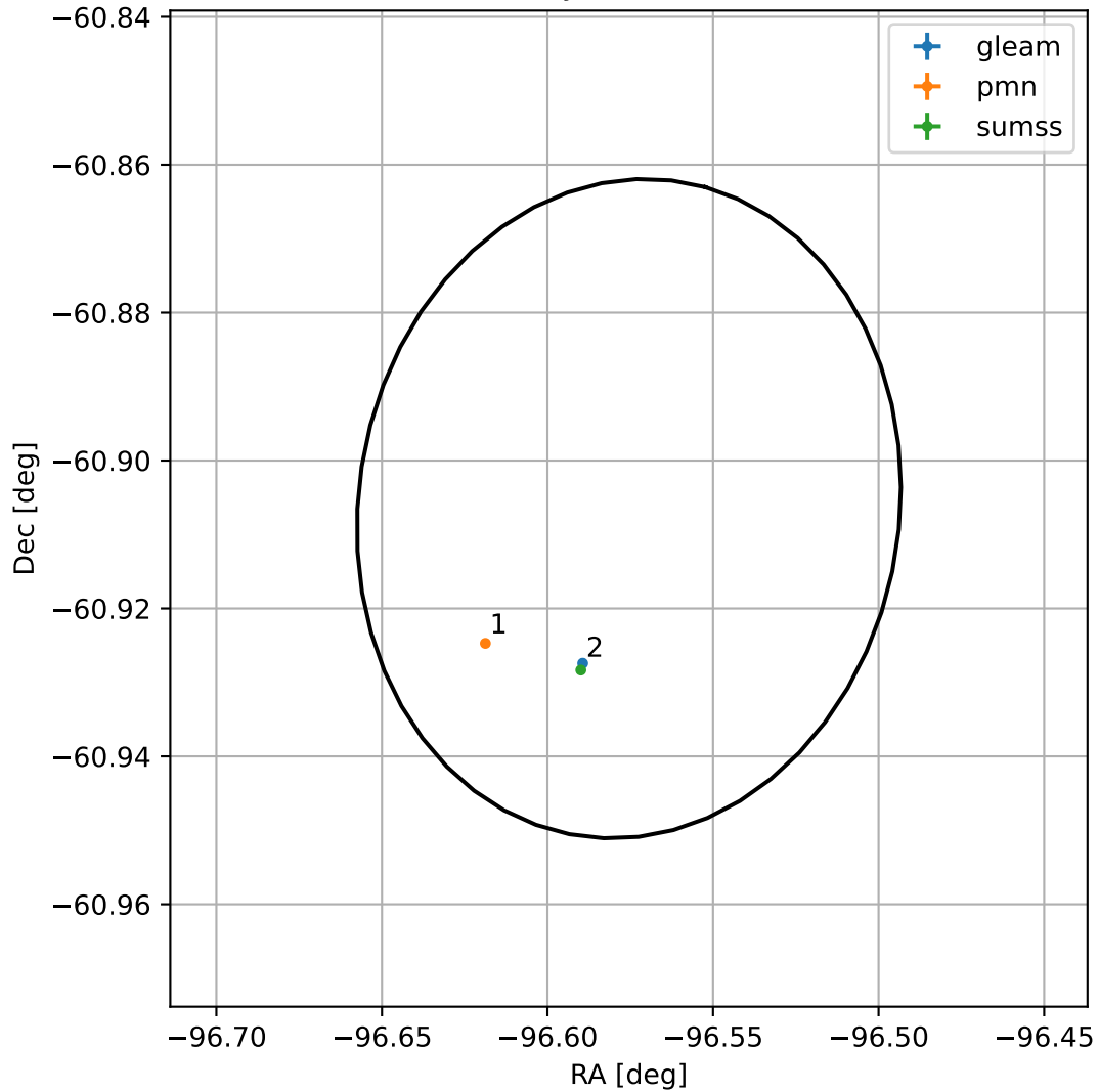
4FGL J1733.6-6054
