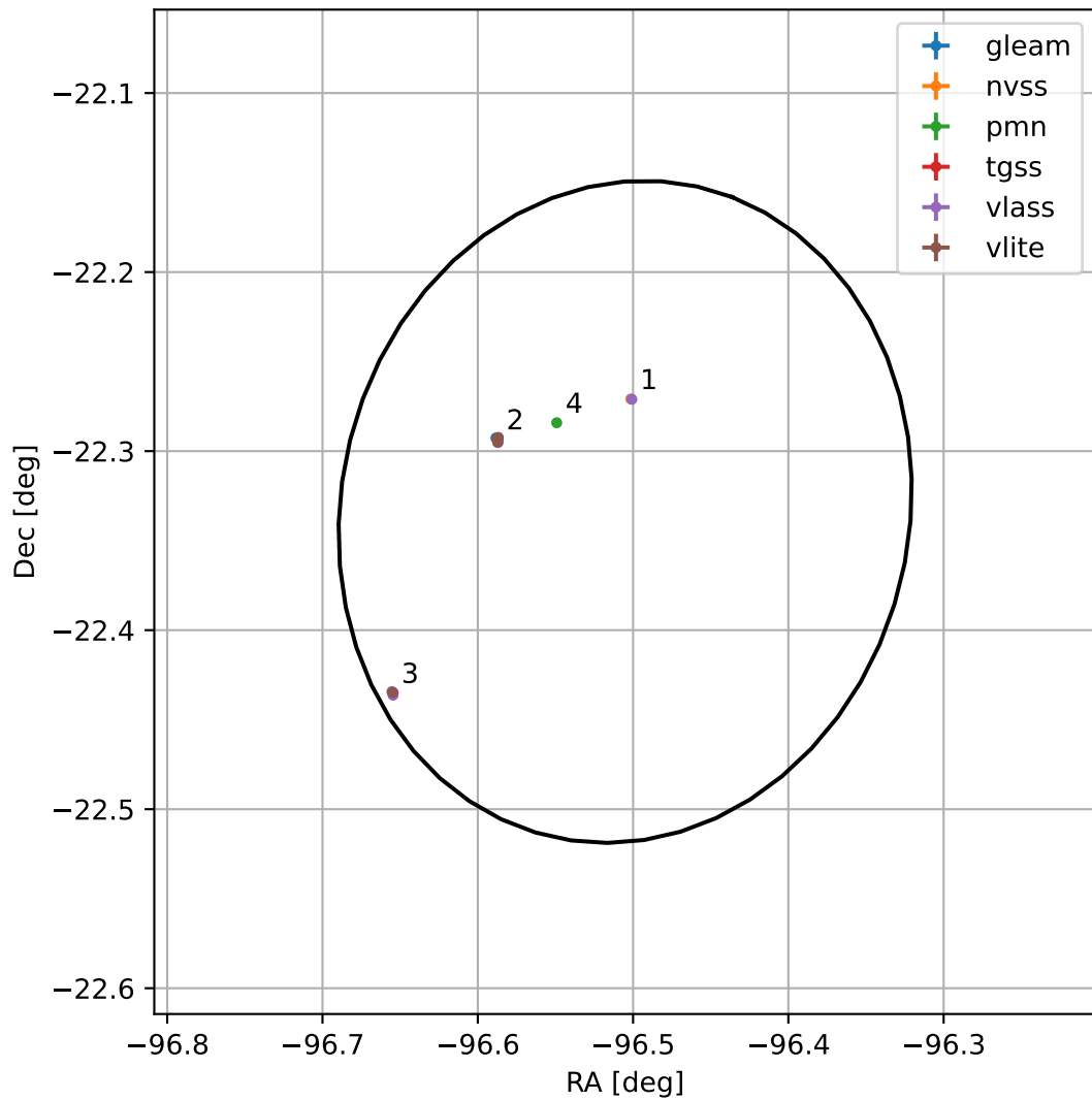
4FGL J1733.9-2220
