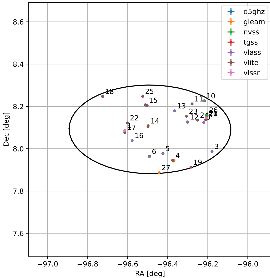
4FGL J1734.0+0805
