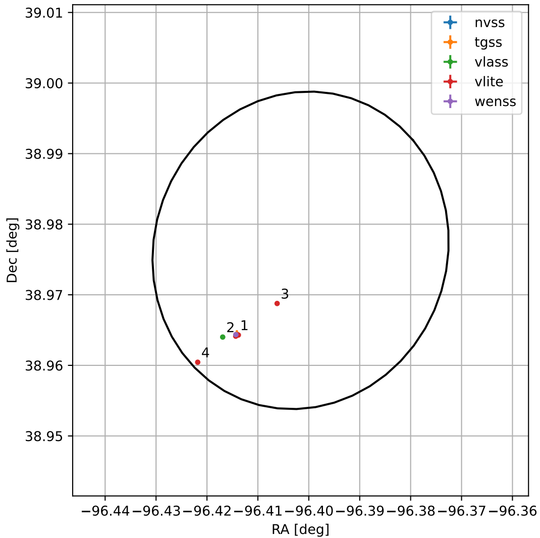
4FGL J1734.3+3858
