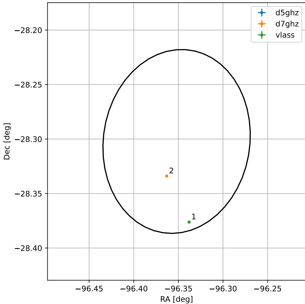
4FGL J1734.5-2818
