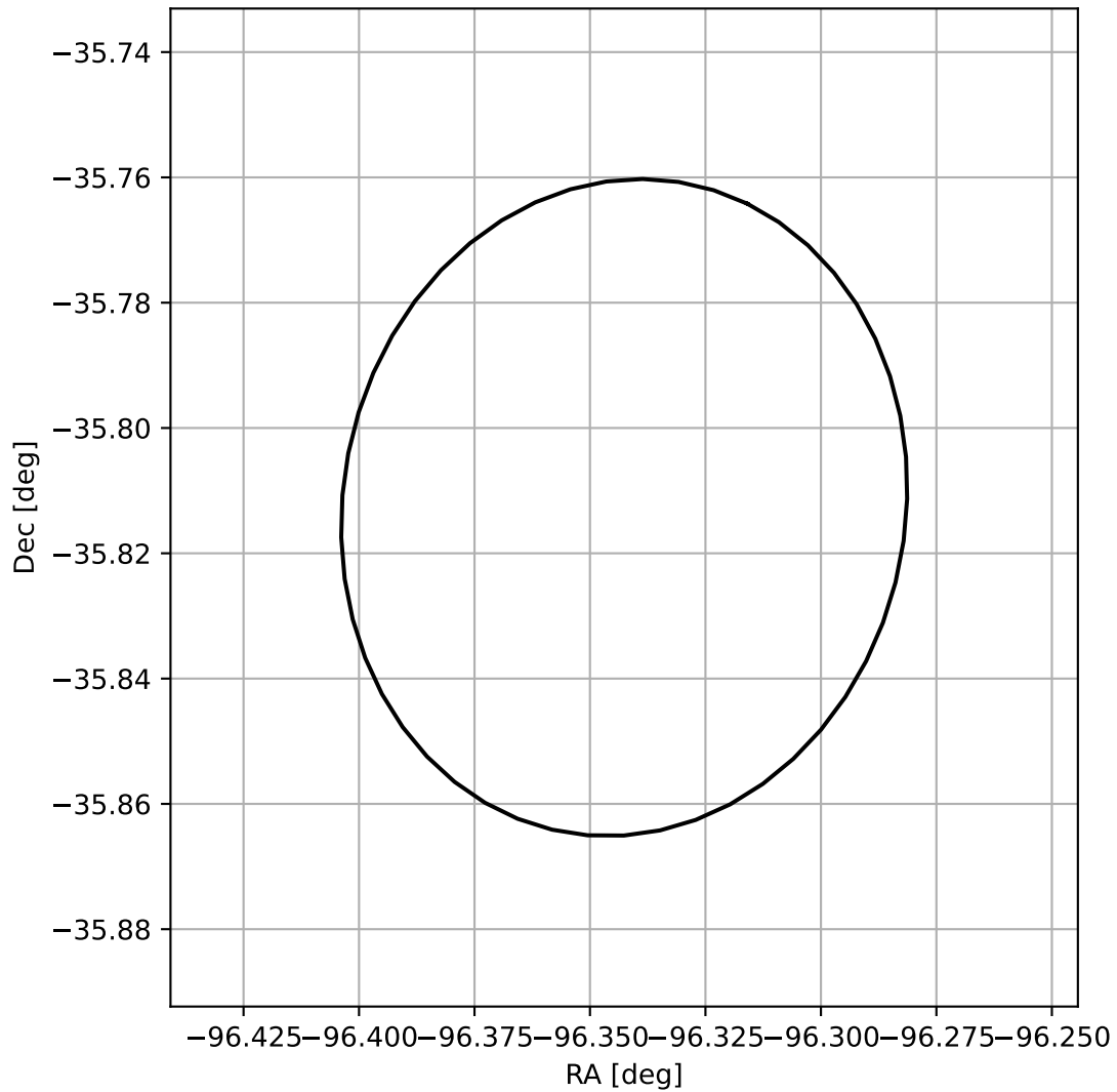
4FGL J1734.6-3548
