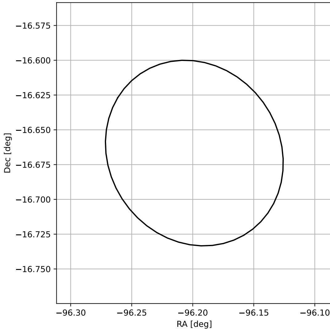
4FGL J1735.2-1640
