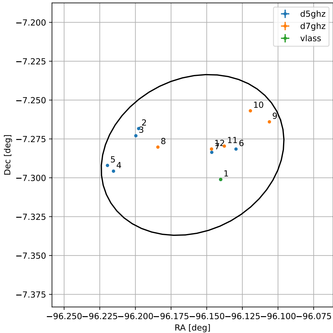
4FGL J1735.3-0717
