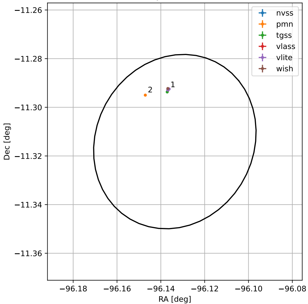
4FGL J1735.4-1118
