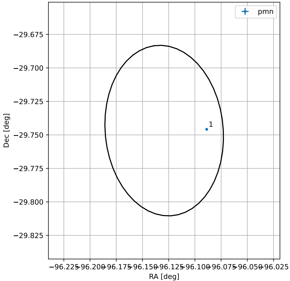
4FGL J1735.4-2944
