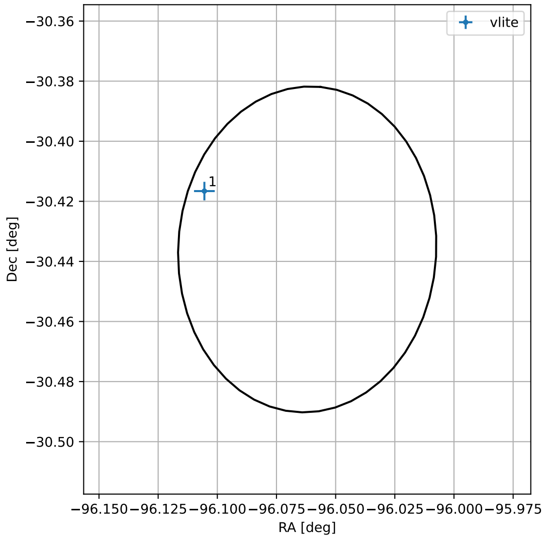
4FGL J1735.7-3026
