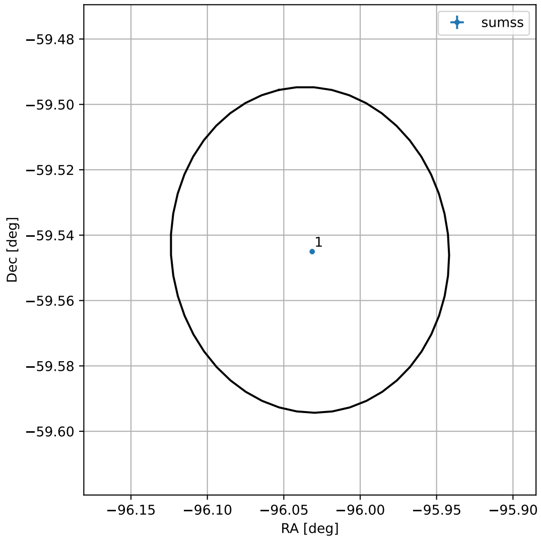
4FGL J1735.8-5932
