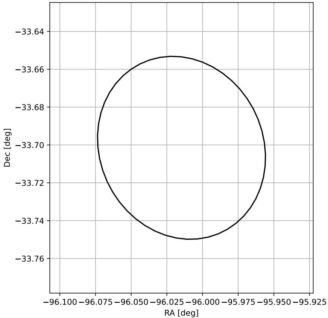
4FGL J1735.9-3342
