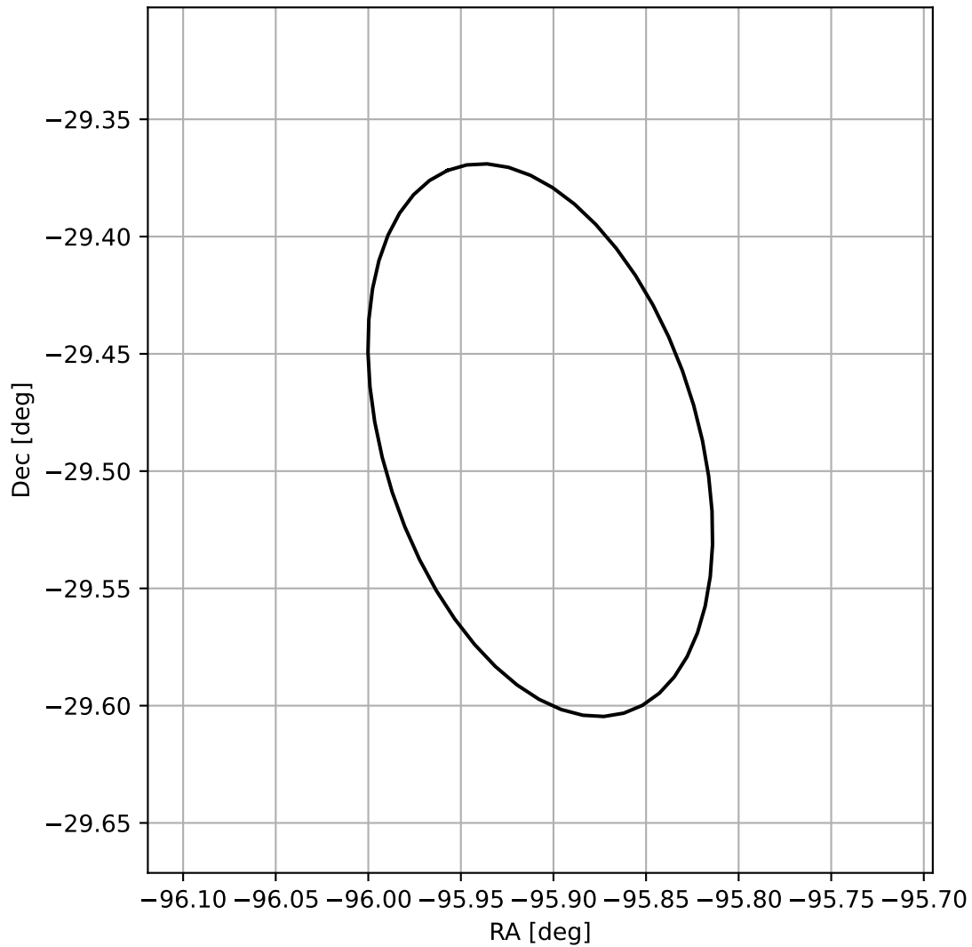
4FGL J1736.3-2929
